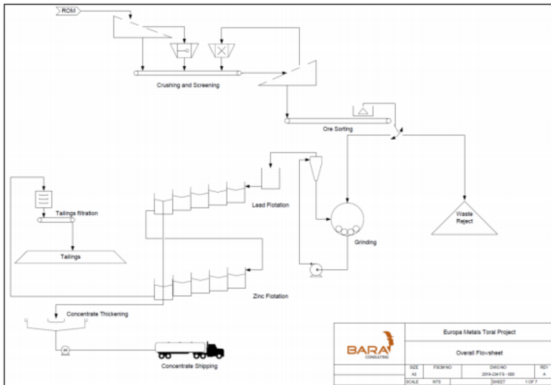
Figure 1: Basic Toral Flowsheet showing comminution, ore sorting, flotation, concentrate handling and dry stack tailings
